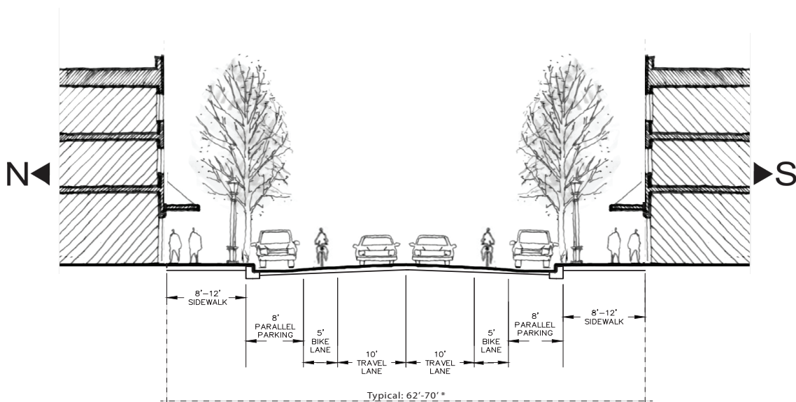
Figure 7-5: Street Cross-Sections Continued, Updated 2016
