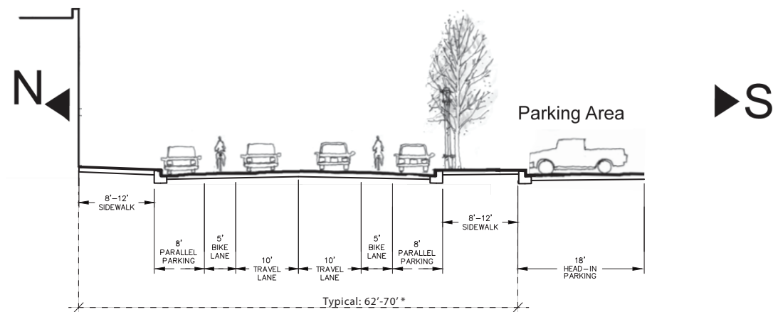
Figure 7-5: Street Cross-Sections Continued, Updated 2016
