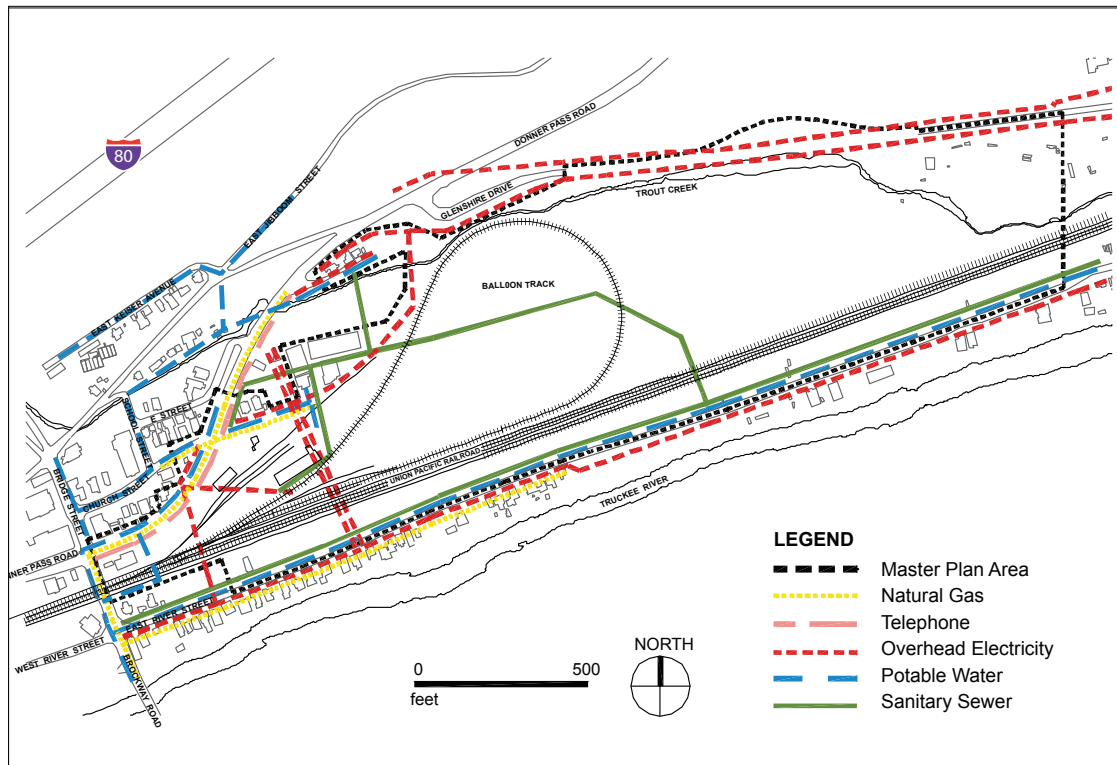
Figure 8-3: Existing Utilities Plan
