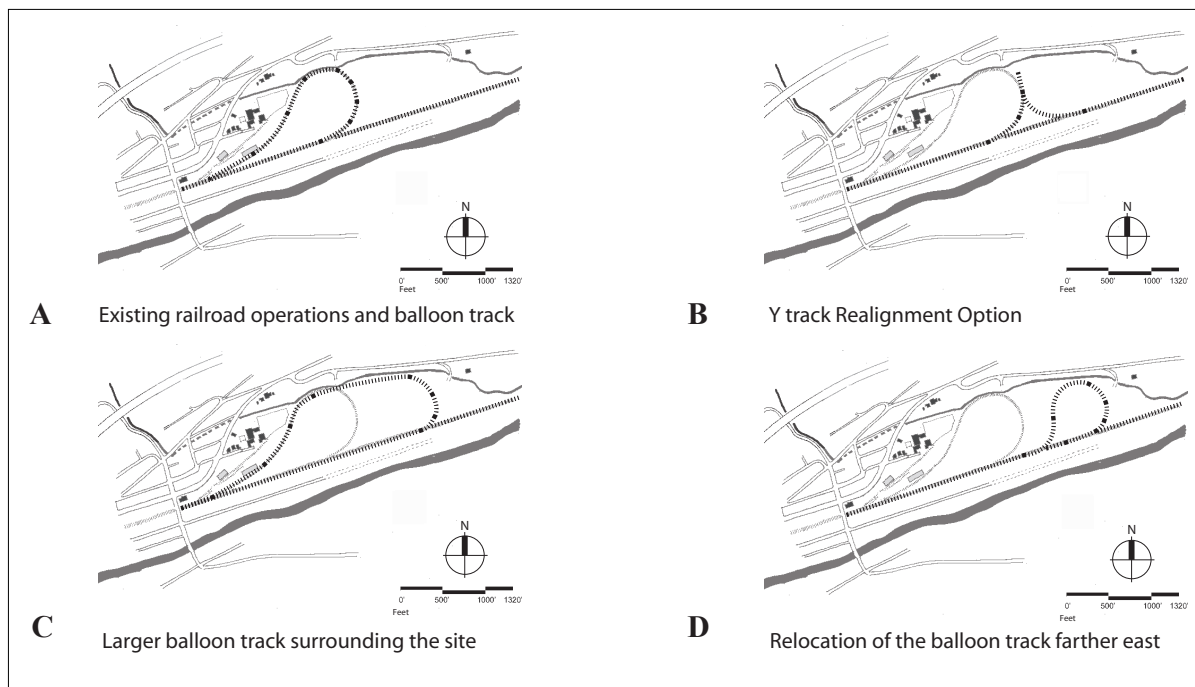
Figure 3-4: Railroad Balloon Track Realignment Options
