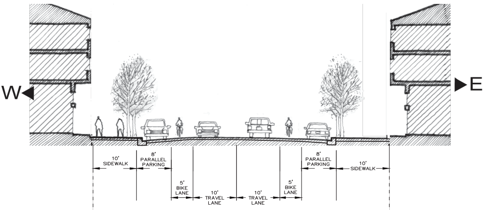
Figure 7-5: Street Cross-Sections Continued, Updated 2016
