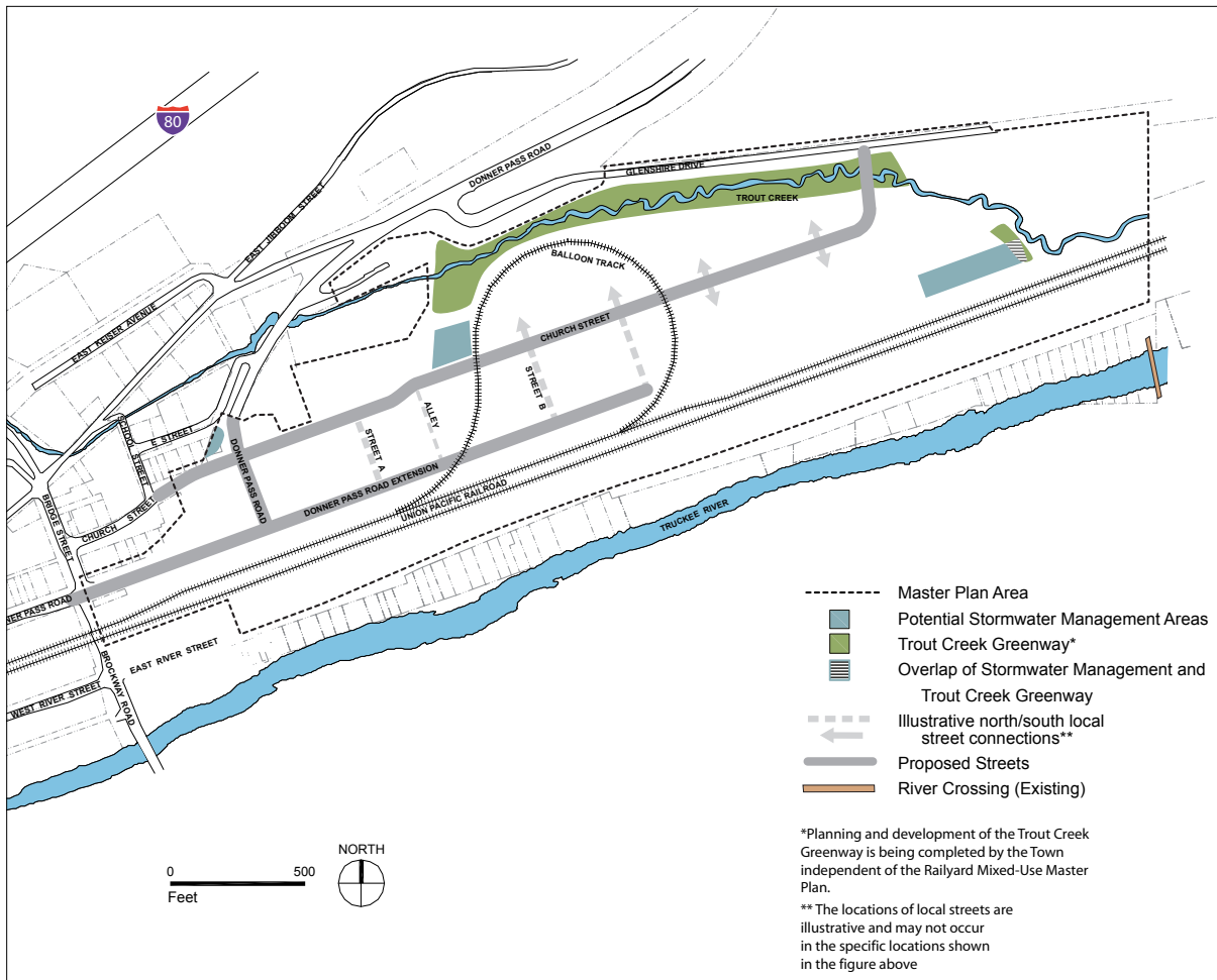
Figure 8-2: Stormwater Concept Plan
